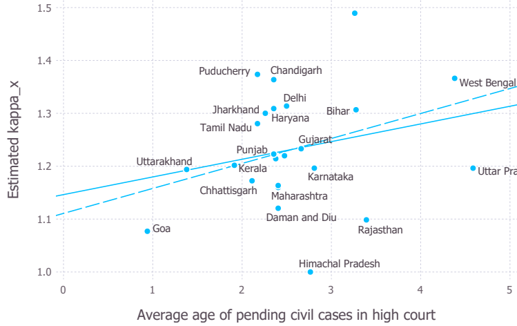
Figure 4 Correlation between 1/\bar{t}_x and court quality
